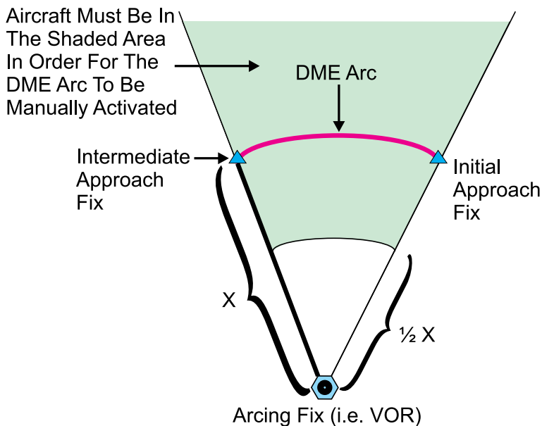
Figure 6-21 DME Arc Example
