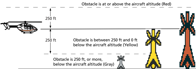
Figure 18-2 HTAWS Obstacle Altitude Correlation
