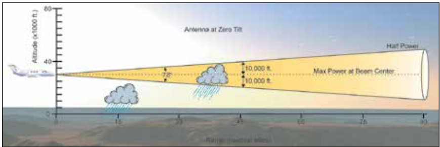
Figure 12-46 Radar Beam from 12 inch Antenna
