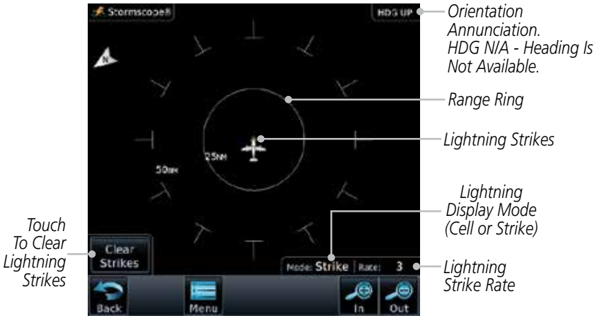
Figure 12-42 StormScope Display (360° Display View Shown)
