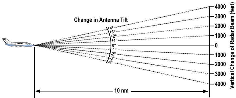
Figure 12-51 Vertical Change in Radar Beam per Nautical Mile
