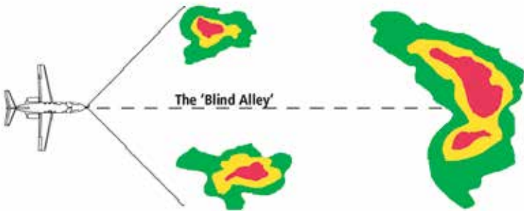
Figure 12-53 The “Blind Alley” Overhead View
